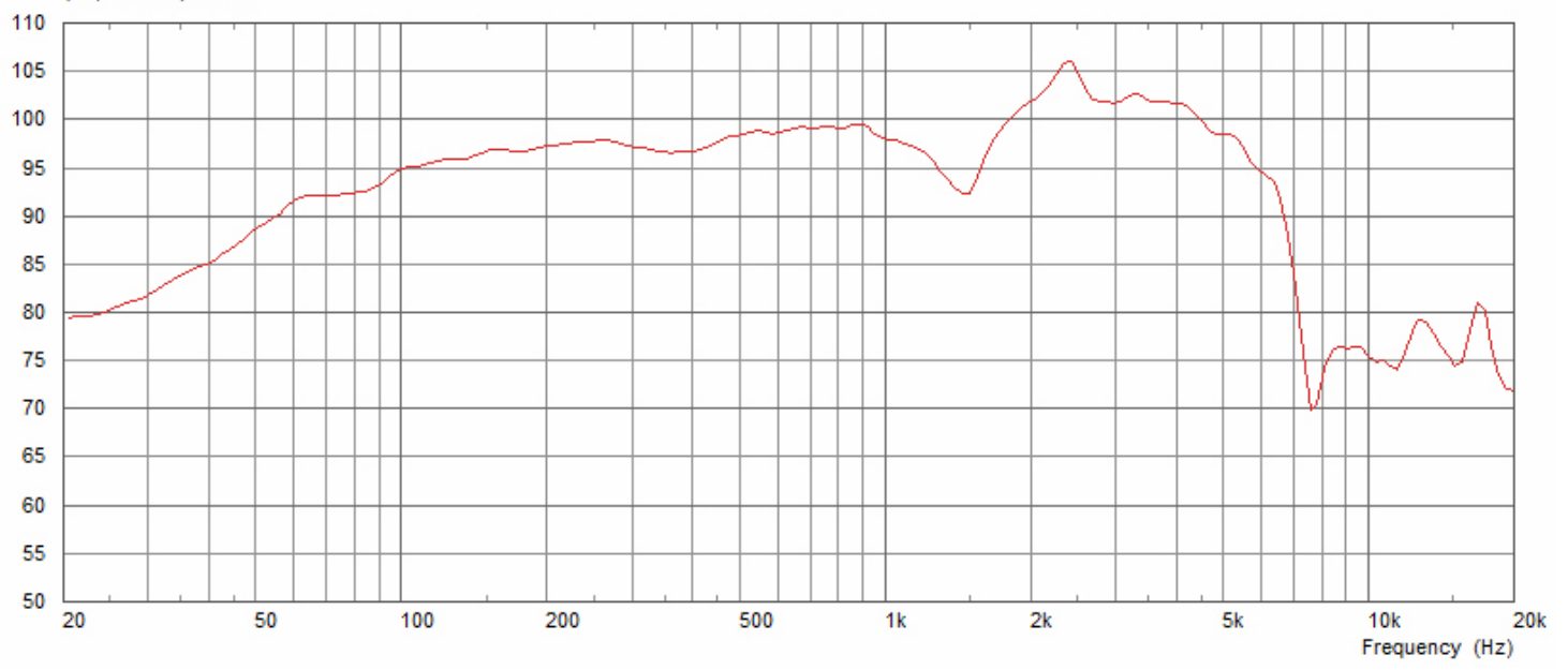
(dB) Sound pressure
